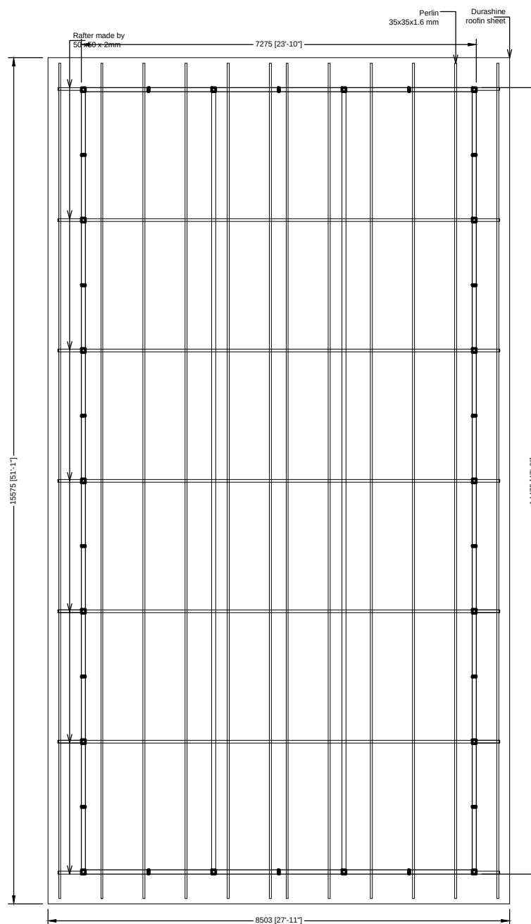
LAYOUT PLAN
