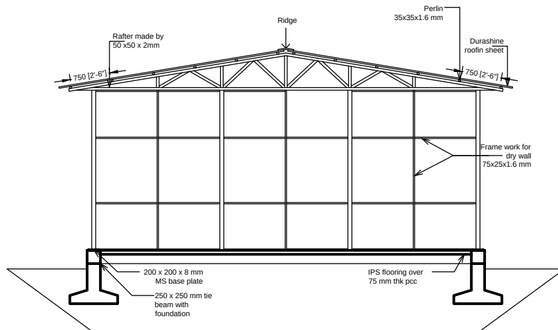
SECTION
